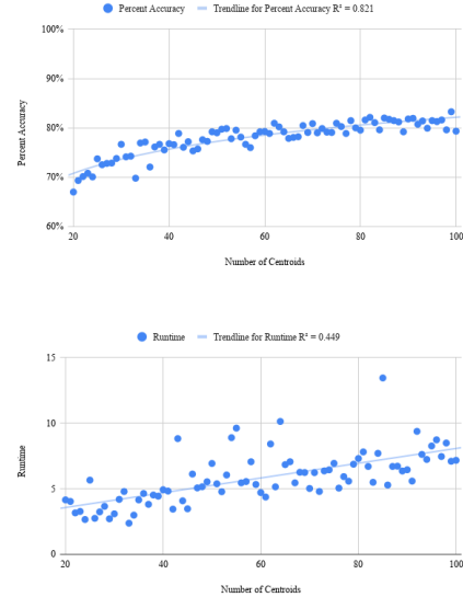
Fig. 1: Effect of increasing the number of centroids on classification accuracy and runtime.
